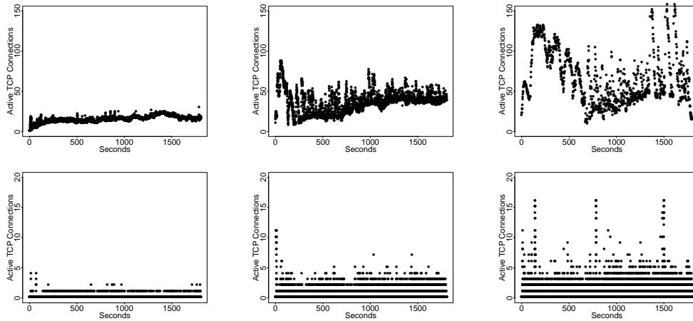
Figure 5: Active TCP Connections for 70 pps (left), 300 pps (middle), and 500 pps (right) (upper: SURGE; lower: SPECweb96).
