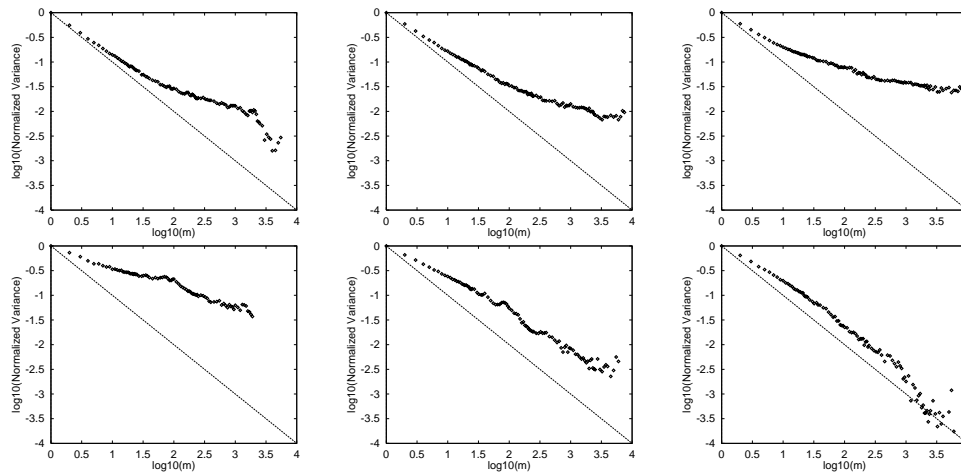
Figure 6: Variance-Time Plots for 70 pps (left), 300 pps (middle), and 500 pps (right) (upper: SURGE; lower: SPECweb96).
